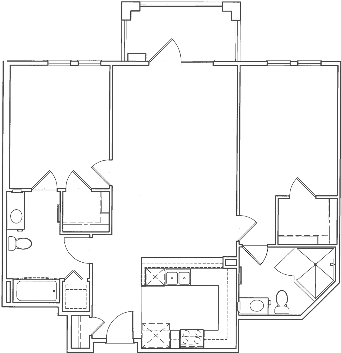
PLAN 3 UNITS #10 & #14 2-BEDROOM
